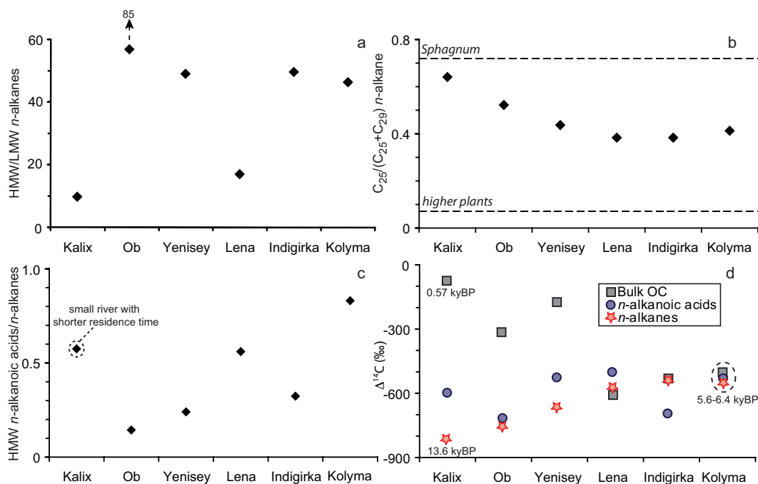
Fig. 2. Molecular and molecular-isotopic patterns of soil marker compounds from west-to-east across the Eurasian Arctic climosequence. (a) Ratio of terrigenous-to-aquatic derived n -alkanes (HMW n -alkanes to LMW n -alkanes). (b) C_{25}/(C_{25}+C_{29}) n -alkane ratio indicating contribution from Sphagnum -rich peatlands to the terrestrial OC (end-member values in Vonk et al., 2009). (c) Ratio of HMW n -alkanoic acids to HMW n -alkanes indicating an increased contribution of less degraded carbon eastward. (d) \Delta^{14}C values of bulk OC, n -alkanoic acids ( C_{24}+C_{26}+C_{28} ) and n -alkanes ( C_{27}+C_{29}+C_{31} ) from estuarine surface sediments across the Eurasian Arctic. Uncertainties are smaller than symbols (see Table 2).
