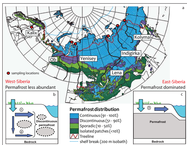
Fig. 1. The Eurasian Arctic with permafrost distributions, studied rivers and possible mechanism of fluvial carbon releases. (a) Permafrost distributions in the Eurasian Arctic (modified from Tarnocai et al., 2009) with Kalix and Russian Arctic rivers (black lines) and sampling locations (red circles). (b) In West-Siberian discontinuous permafrost, top soils (transport route 1) deliver bulk organic carbon (OC) with relatively young ^{14}\text{C} while groundwater and thermokarst-related transport (transport route 2) delivers more refractory, older OC. (c) Continuous permafrost in East-Siberia restricts carbon transport predominantly to the active layer (transport route 3) causing release of bulk OC and refractory lipids of similar ^{14}\text{C} age.
