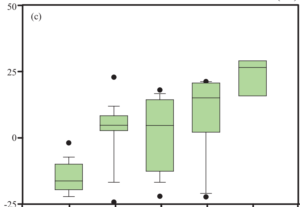
\Delta\delta^{13}\text{C} C16:1 \omega 5c relative to source methane (‰)
