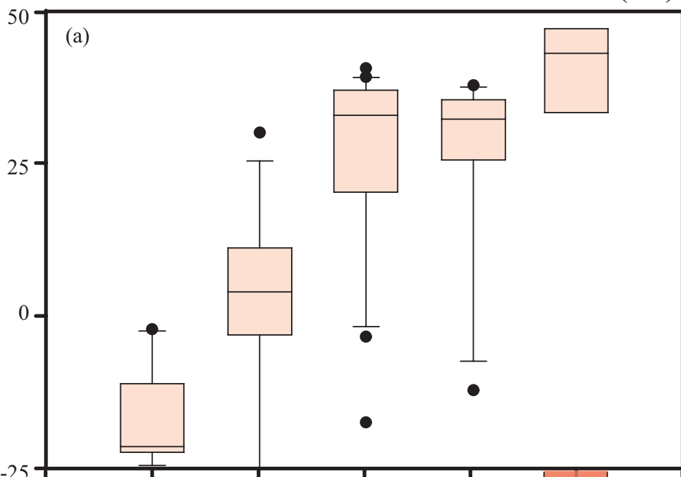
\Delta\delta^{13}\text{C} archaeol relative to source methane (‰)
