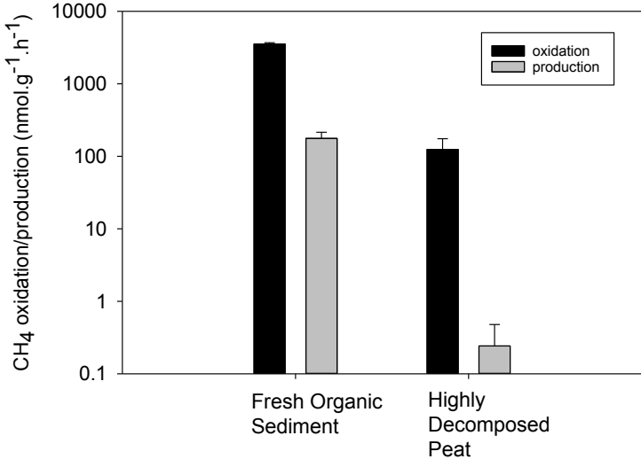
Figure S1: Incubation data from Zarnekow, a freshwater minerotrophic fen in Northeastern Germany. Rates of methane production (n=3) and methane oxidation (n=3) are shown for both fresh (surficial) organic sediment and the bulk peat.
