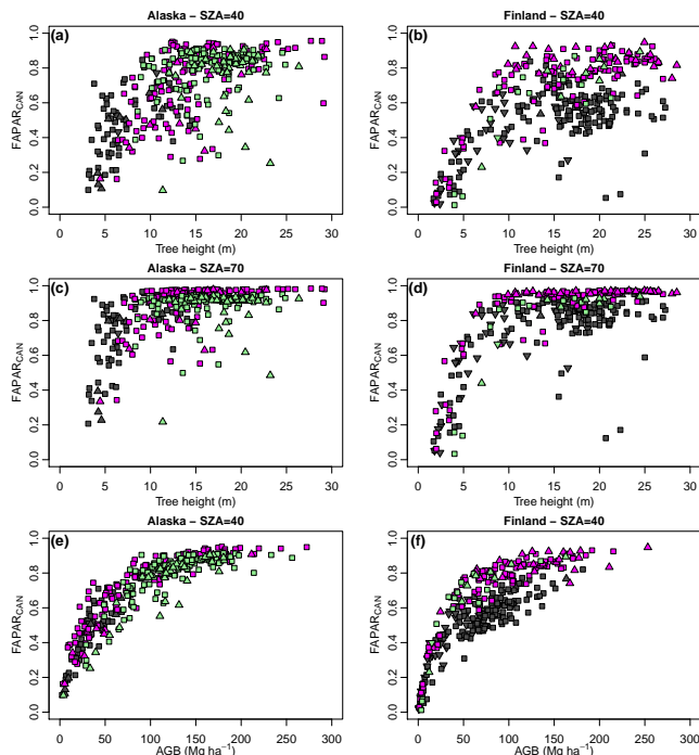
Figure 5. Black-sky FAPAR_{CAN} as a function of tree height (a–d) and AGB (e–f). Relations to tree height are shown for two SZAs, 40^\circ (a–b) and 70^\circ (c–d), representing solar noon at midsummer and the annual average in the study regions. Left hand column shows the results for the Alaskan data, and right hand column for the Finnish data. The figures show only monospecific plots, i.e., plots in which the basal area proportion of one of the species exceeded 80%. For explanation of the symbols, see legend in Fig. 4.
