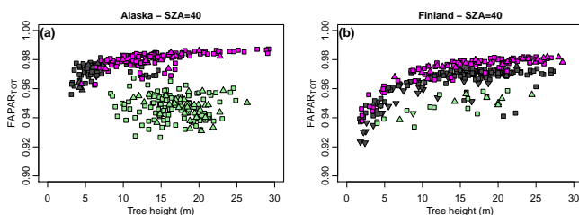
Figure 6. FAPAR_{TOT} as a function of tree height at SZA of 40^\circ . The figures show only monospecific plots, i.e., plots in which the basal area proportion of one of the species exceeded 80%. For explanation of the symbols, see legend in Fig. 4.
