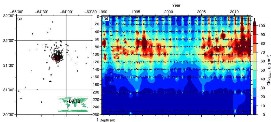
Figure 1. Horizontal (a) and vertical (b) distribution of pigment measurements taken at BATS (black dots) overlaid on a contour plot of HPLC-measured Chl a hapto at BATS. The red box in (a) shows the PIC grid cell containing the most BATS measurements (PIC data shown in Fig. 8), while the black box in (b) shows the upper 30 m of measurements used for PIC-Chl a hapto correlations and correlations presented in Fig. 3.
