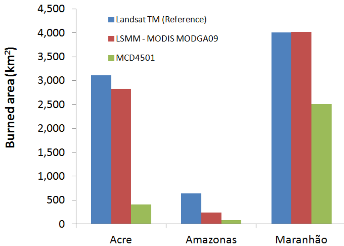
Figure S1: Comparison of the Landsat TM, LSMM – MODIS MODGA09 and MCD4501 burnt area products
